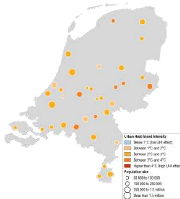
Figure 20: Urban heat island intensity index, 2021
