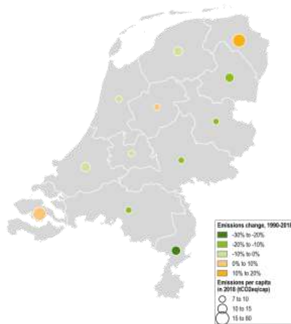
Figure 18: Change in production-based emissions in large regions, 1990-2018
