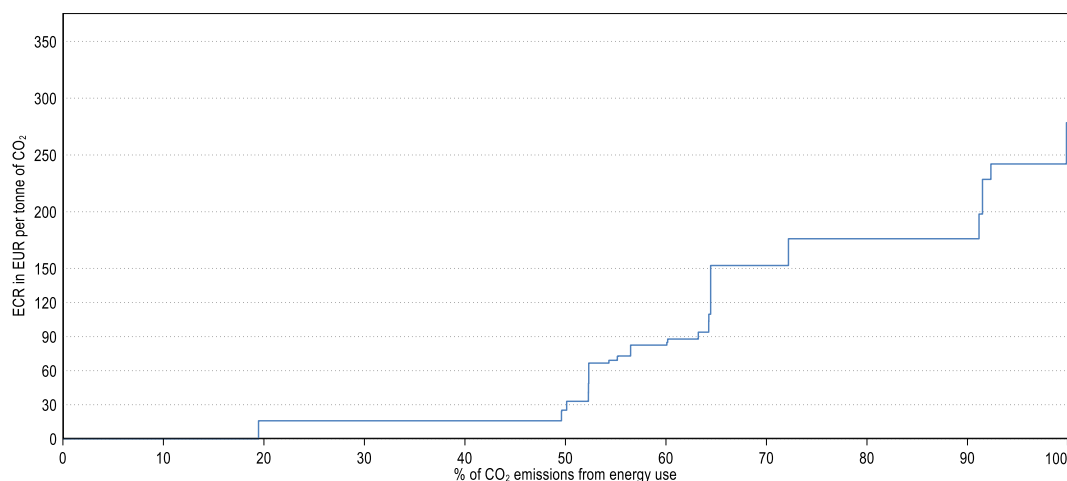
Figure 1. Proportion of CO 2 emissions from energy use subject to different levels of effective carbon rates in Slovenia in 2018
