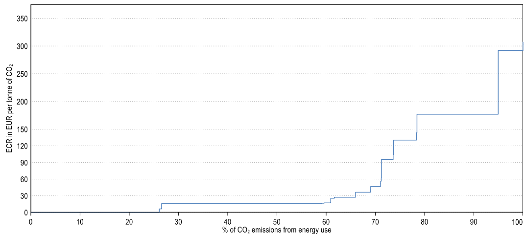
Figure 1. Proportion of CO 2 emissions from energy use subject to different levels of effective carbon rates in Portugal in 2018
