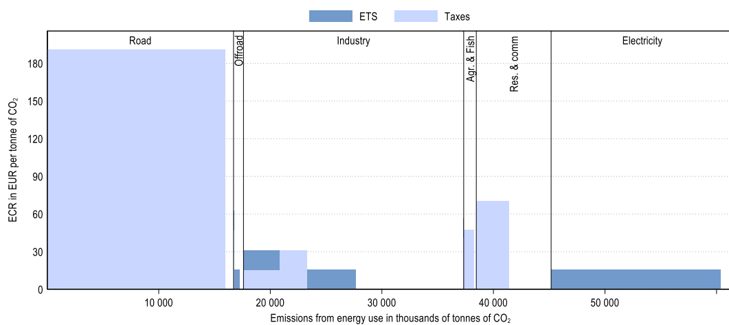
Figure 2. Average effective carbon rates in Portugal by sector and component in 2018
