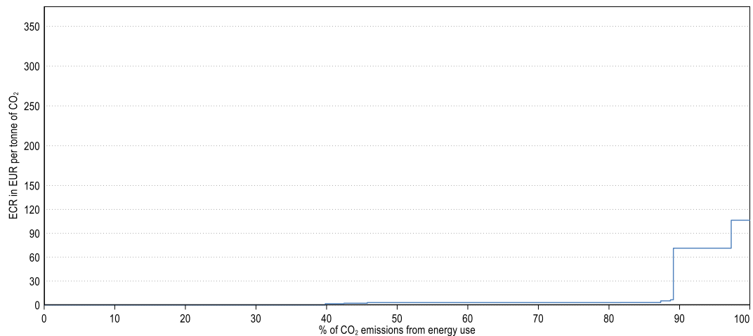
Figure 1. Proportion of CO 2 emissions from energy use subject to different levels of effective carbon rates in India in 2018
