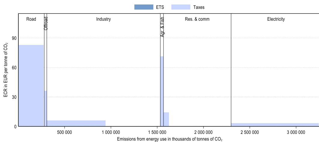
Figure 2. Average effective carbon rates in India by sector and component in 2018
