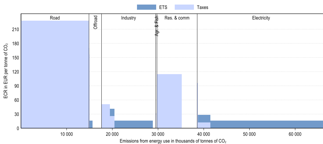
Figure 2. Average effective carbon rates in Greece by sector and component in 2018
