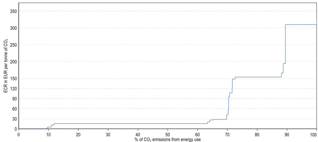
Figure 1. Proportion of CO 2 emissions from energy use subject to different levels of effective carbon rates in Greece in 2018
