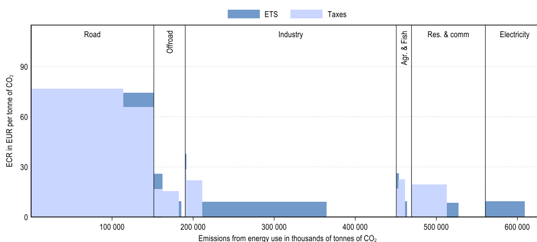
Figure 2. Average effective carbon rates in Canada by sector and component in 2018
