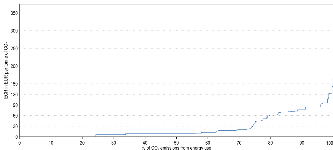
Figure 1. Proportion of CO 2 emissions from energy use subject to different levels of effective carbon rates in Canada in 2018
