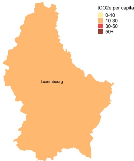
Figure 1. Estimated regional greenhouse gas emissions per capita Tons CO 2 equivalent (tCO 2 e), large regions (TL2), 2018
