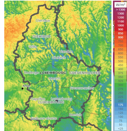
Figure 7. Wind power potential Mean wind power density (W/m 2 )
