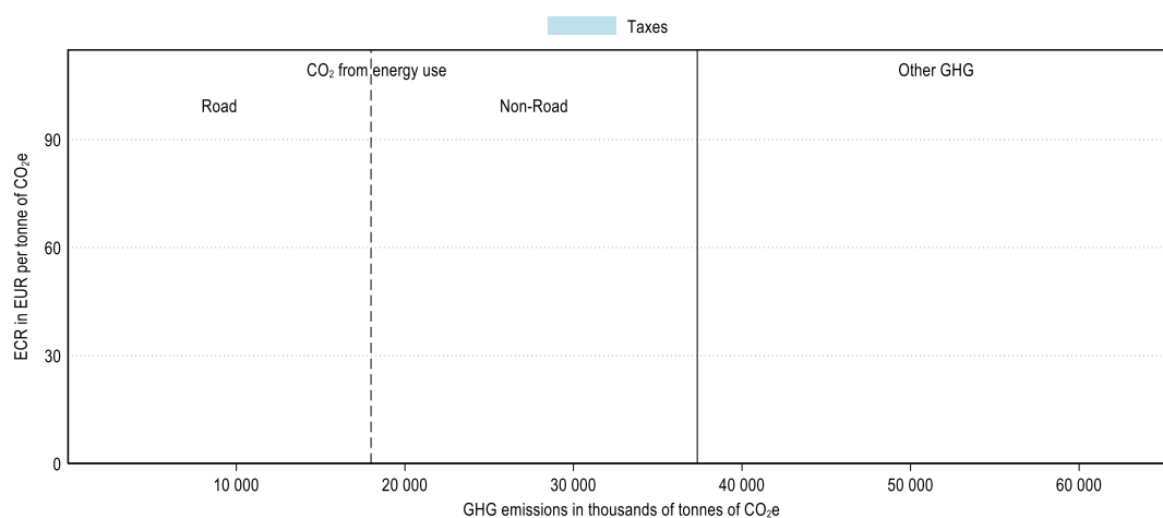
Figure 2. Average effective carbon rates in Ecuador by sector and component in 2021
