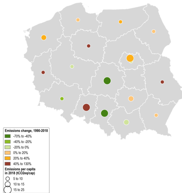
Figure 18: Change in production-based emissions in large regions, 1990-2018
