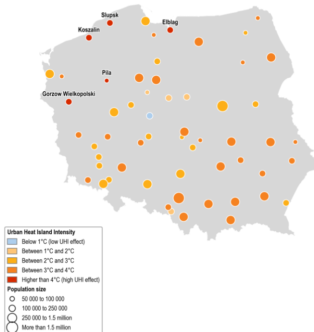
Figure 20: Urban heat island intensity index, 2021
