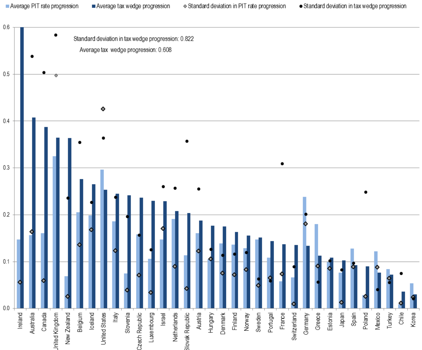
Figure S.7: Overall average PIT rate and tax wedge progression and standard deviation across 5 income intervals 1 A. For one-earner married couples with 2 children, income ranging from 50% to 200% of the AW
